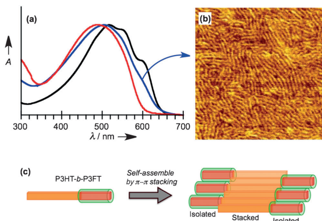
Figure 5. a) Normalized absorption spectra of P3HT (black), P3FT (red), and P3HT(75)- b -P3FT(25) (blue) in their film forms. b) AFM image of the microphase separation of P3HT(75)- b -P3FT(25) (700 nm \times 700 nm; see Figure S18 in the Supporting Information for an image of a larger area). c) Illustration of the plausible self-assembled structure.
